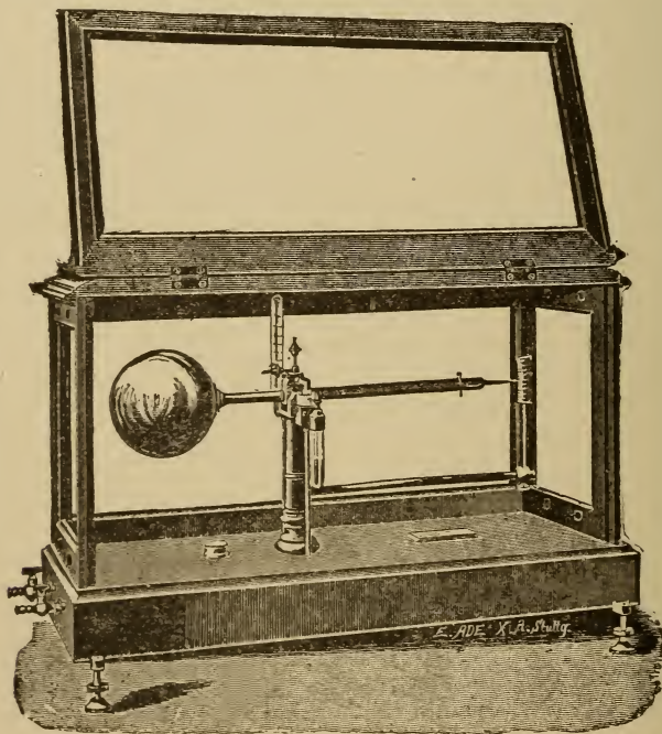
Fig. 84. LUX'S BALANCE FOR WEIGHING GASES.
